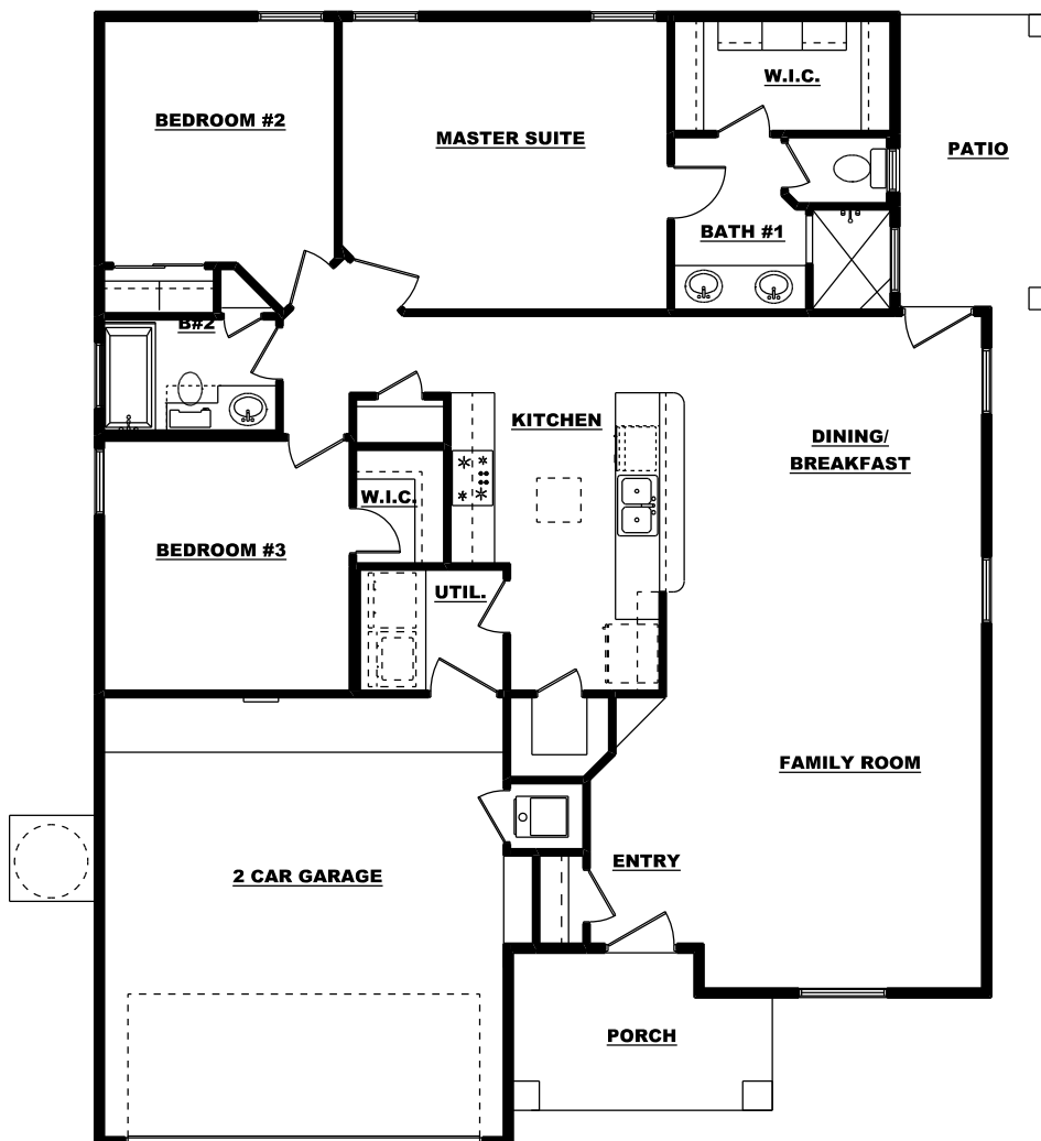
FLOOR PLAN
