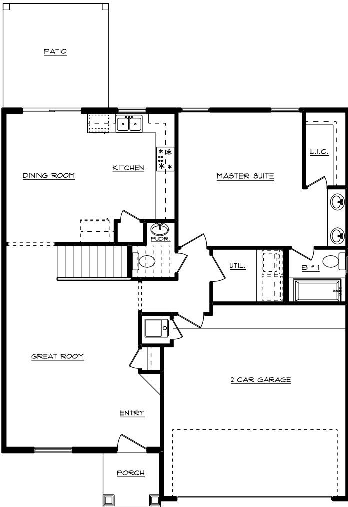
FIRST FLOOR TILE PLAN
