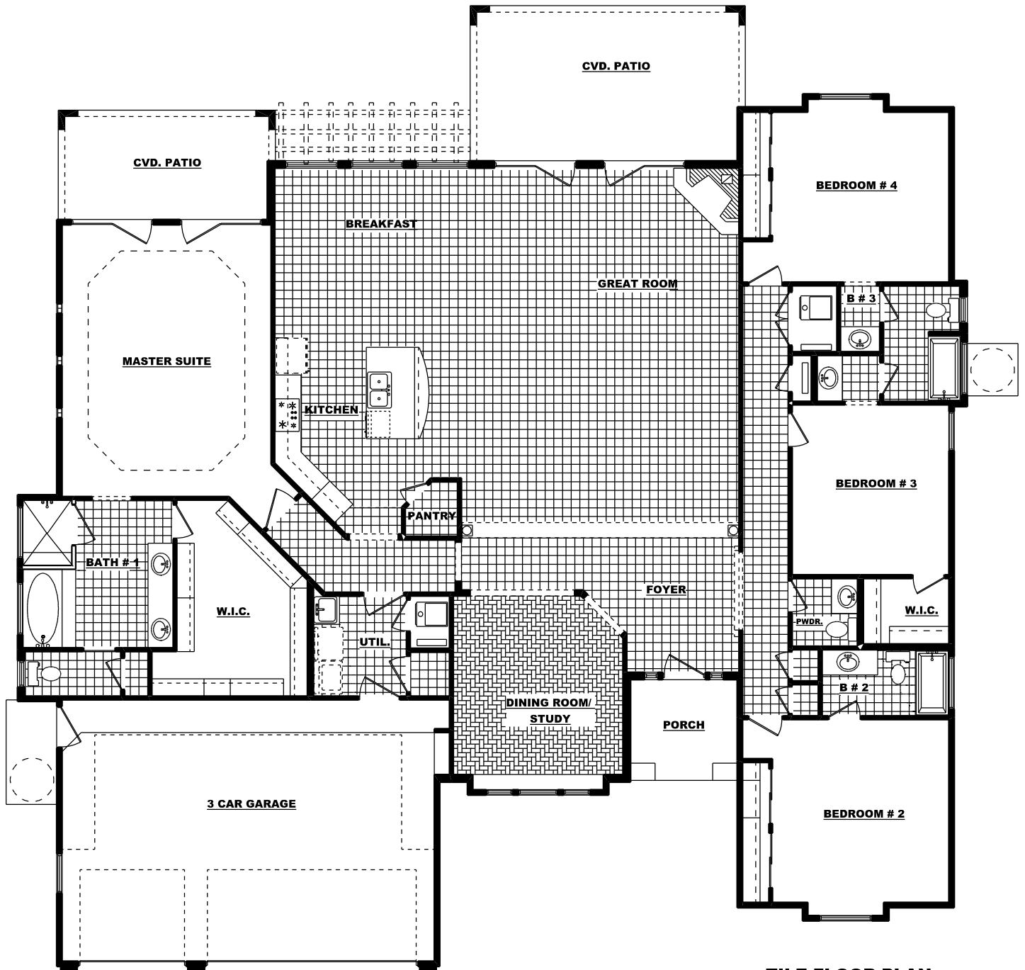
TILE FLOOR PLAN
