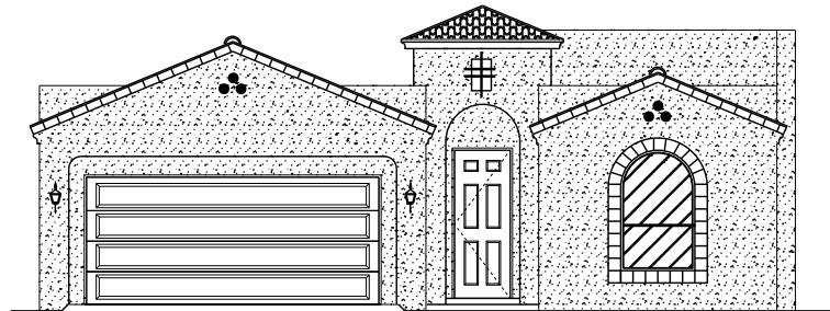
FRONT ELEVATION
