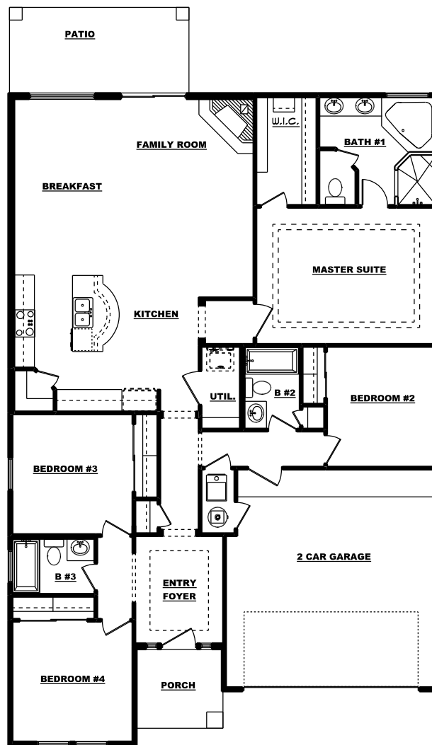
FLOOR PLAN
