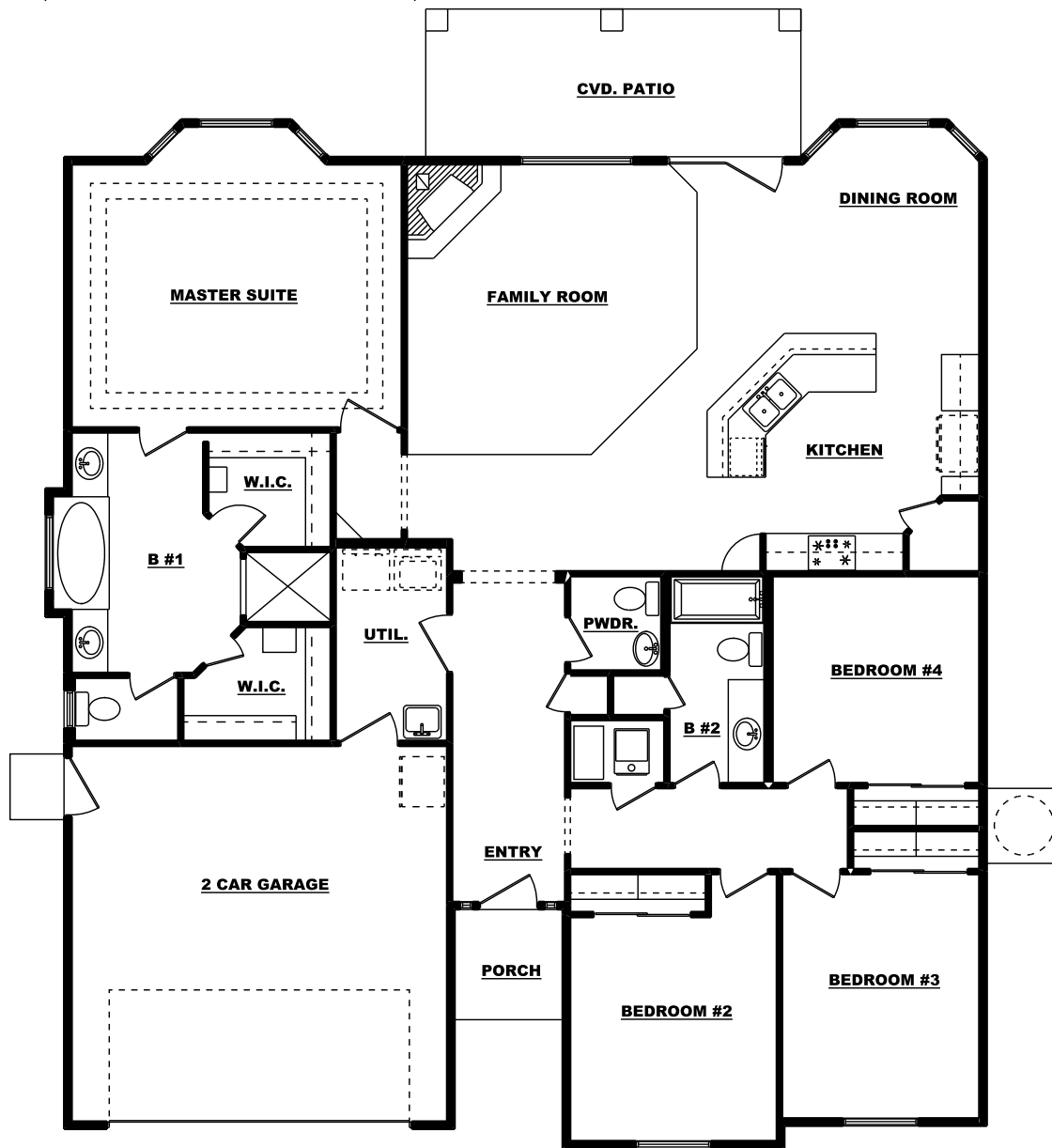
FLOOR PLAN
