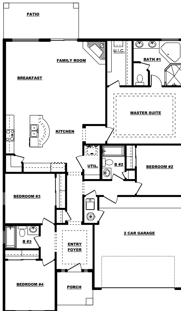
FLOOR PLAN
