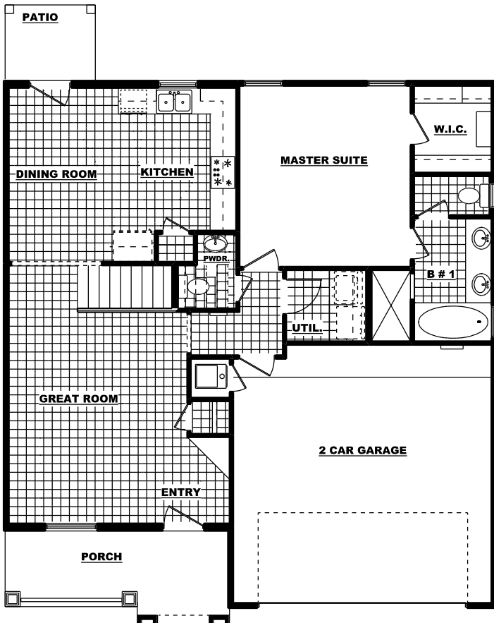
FIRST FLOOR TILE PLAN
