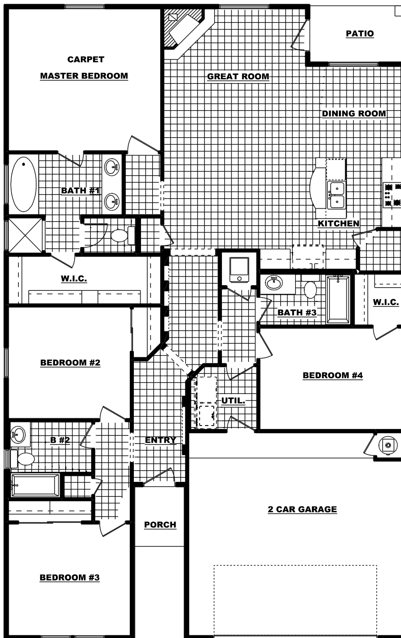
TILE FLOOR PLAN
