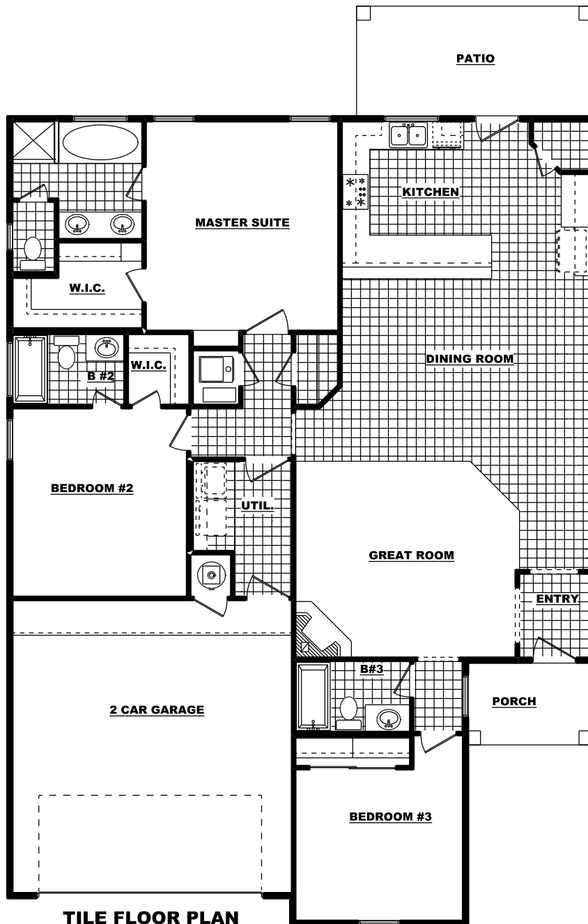
TILE FLOOR PLAN
