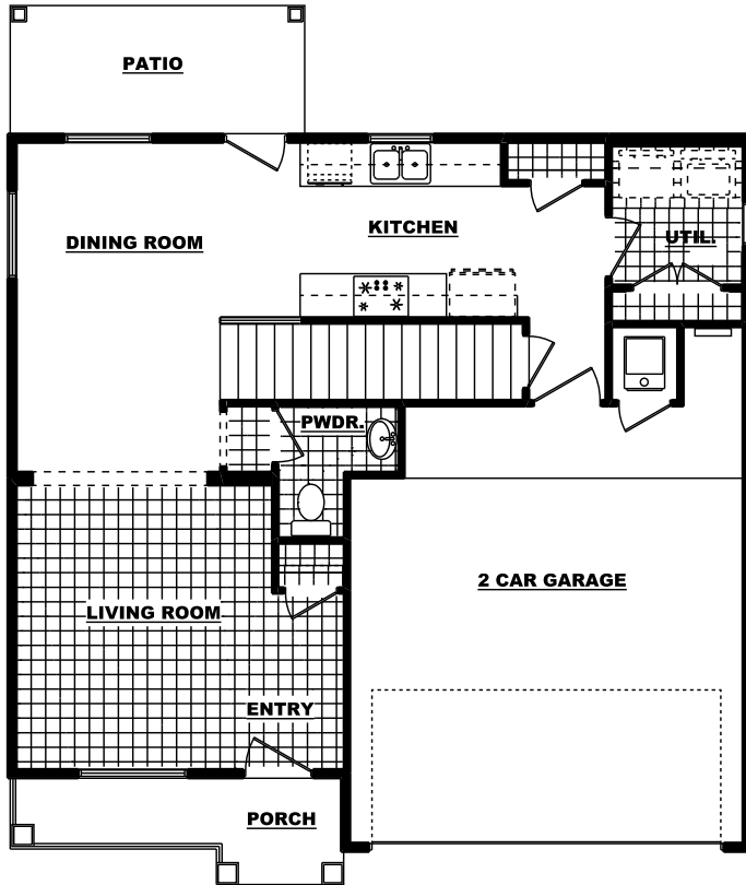
FIRST FLOOR TILE PLAN
