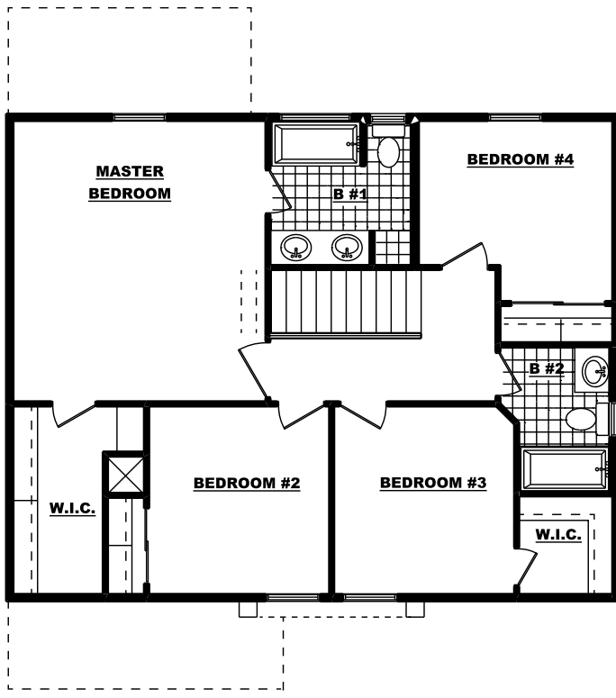
SECOND FLOOR TILE PLAN
