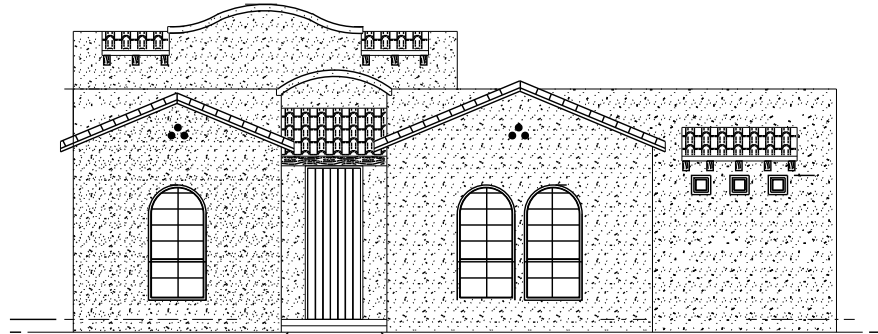
FRONT ELEVATION A
