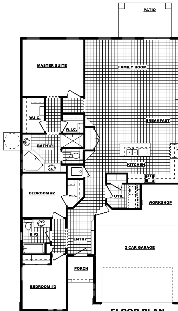
FLOOR PLAN
