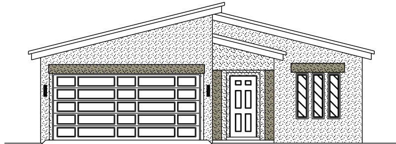
FRONT ELEVATION
