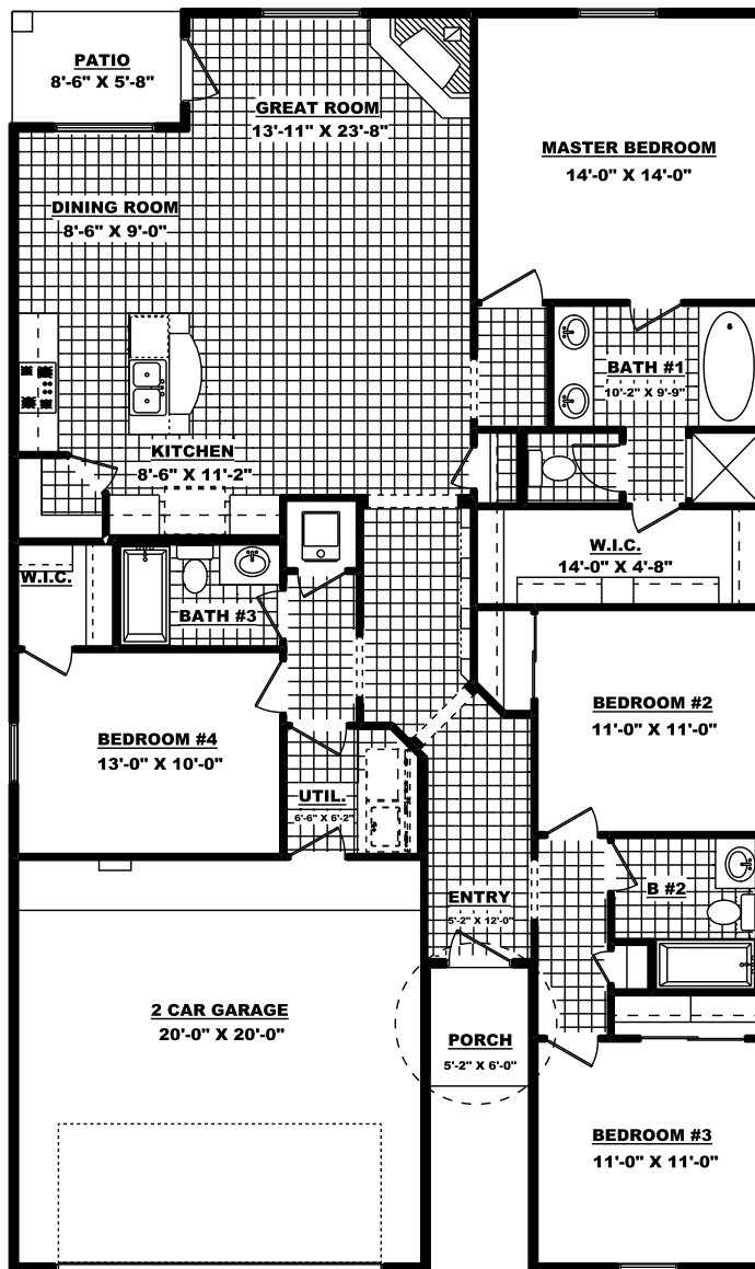
FLOOR PLAN
