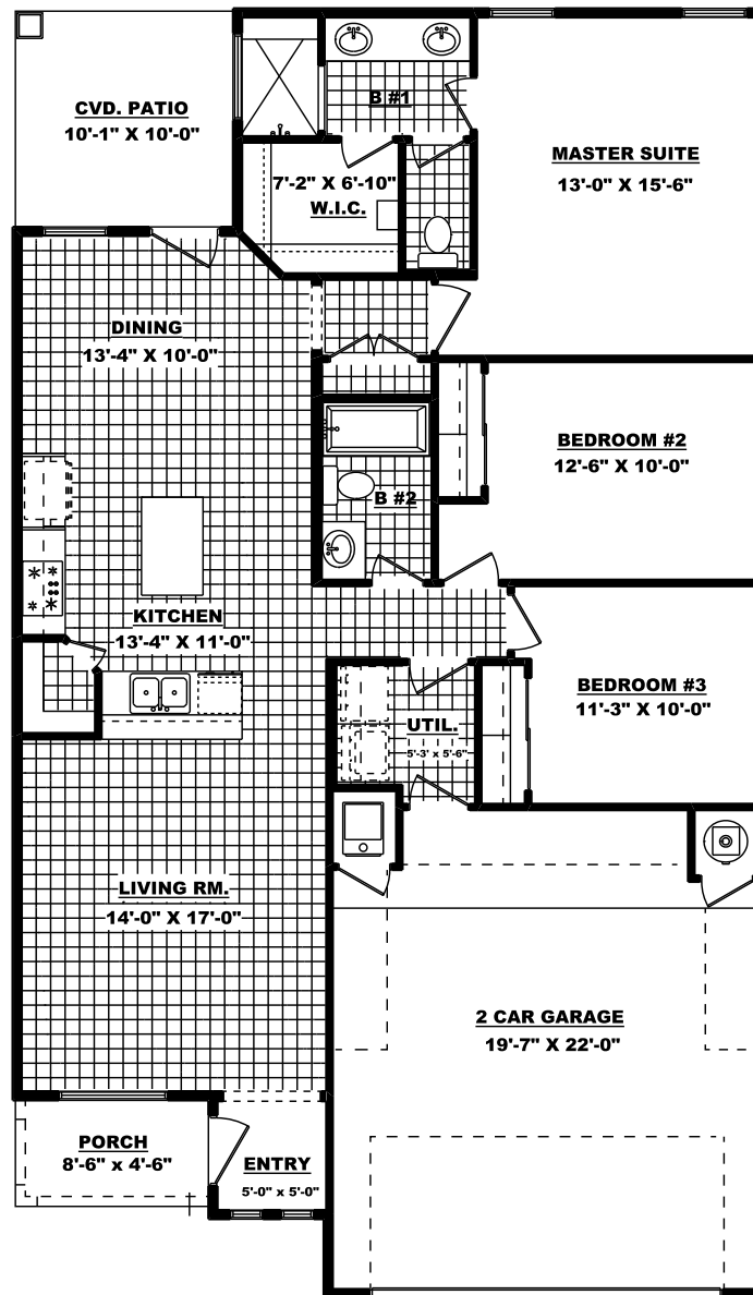
FLOOR PLAN
