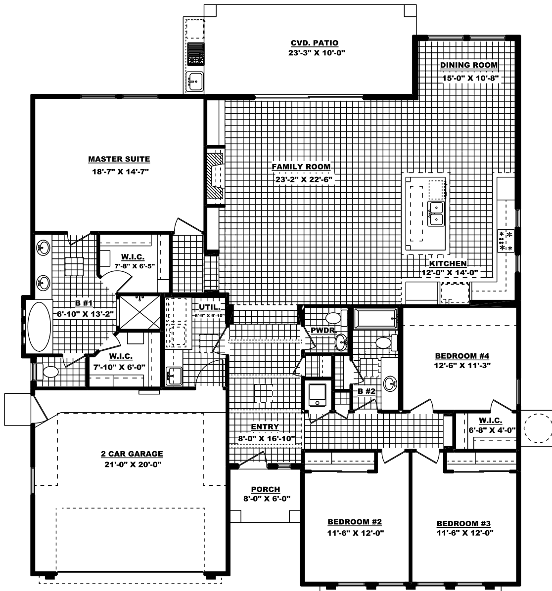
FLOOR PLAN
