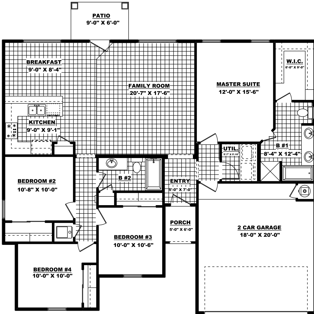
FLOOR PLAN
