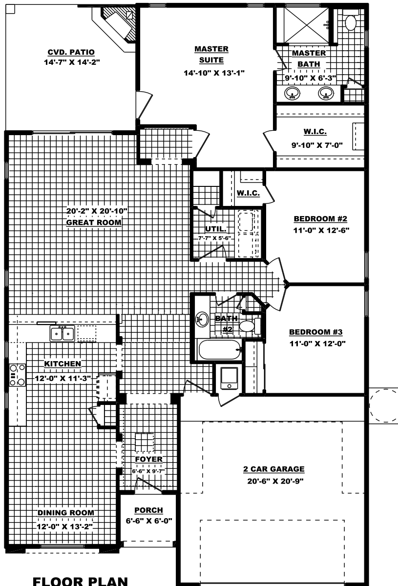
FLOOR PLAN
