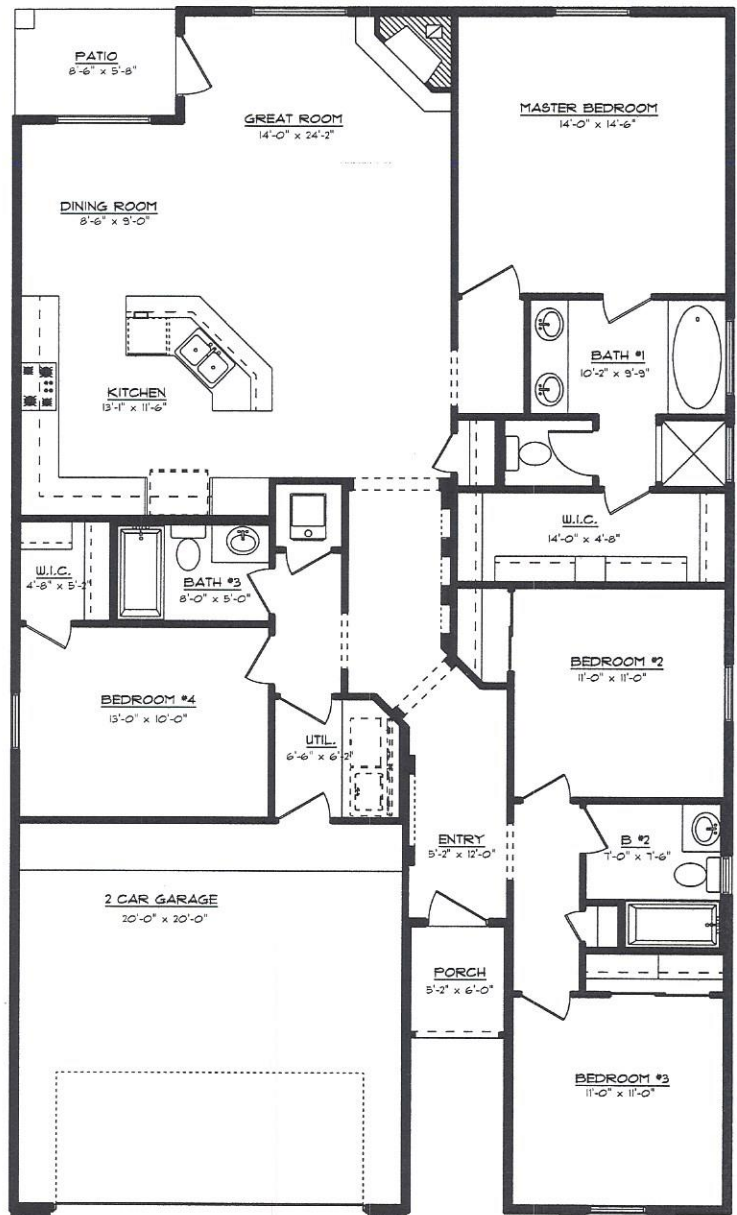
FLOOR PLAN W 37'-4" X D 62'-10"
