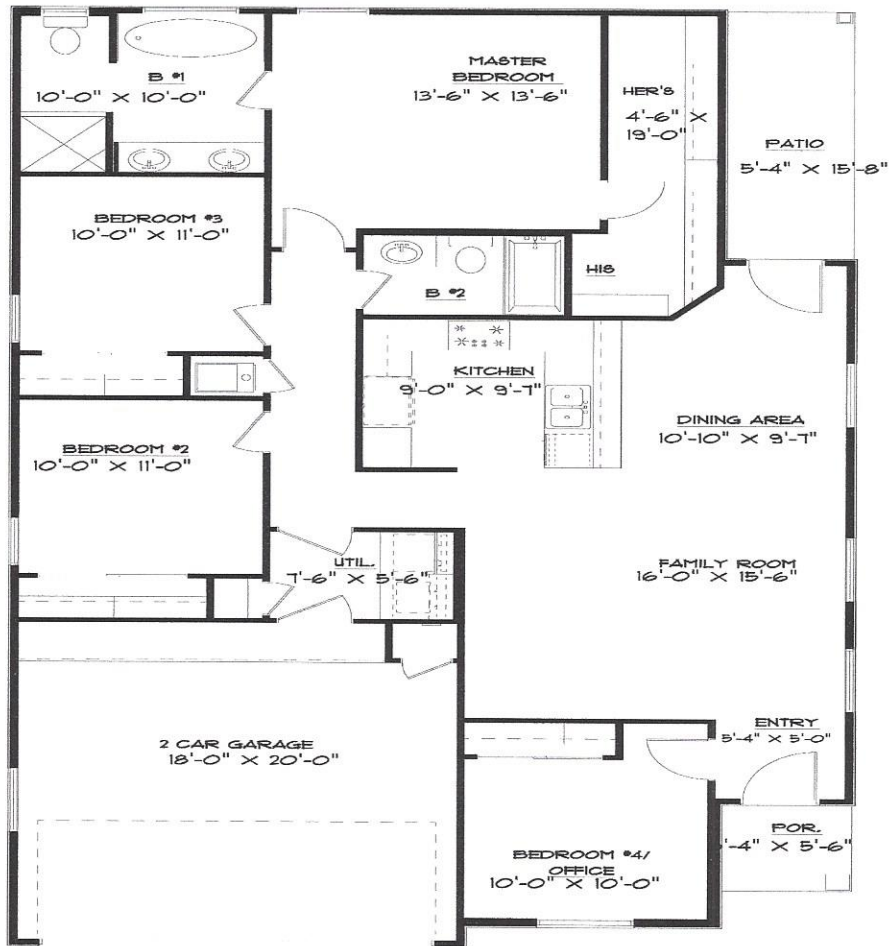
FLOOR PLAN W 34'-6" X D 59'-0"
