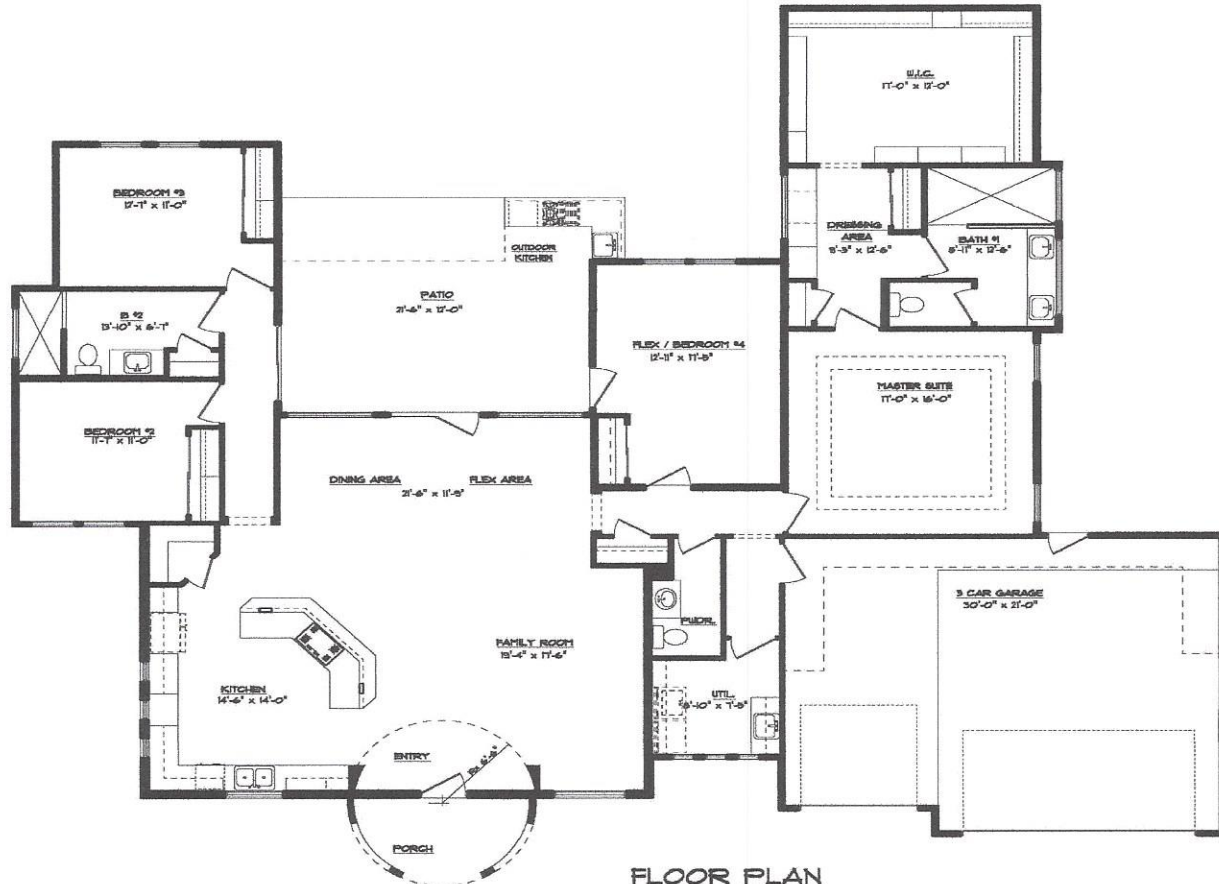
FLOOR PLAN 83'-4" x 65'-0"
