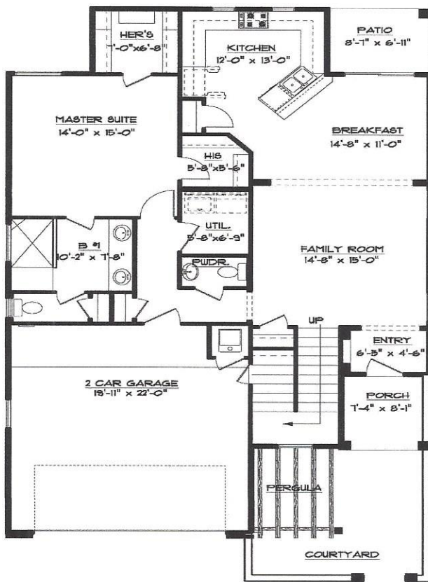
FIRST FLOOR PLAN 35'-6" x 56'-1 1/2"
