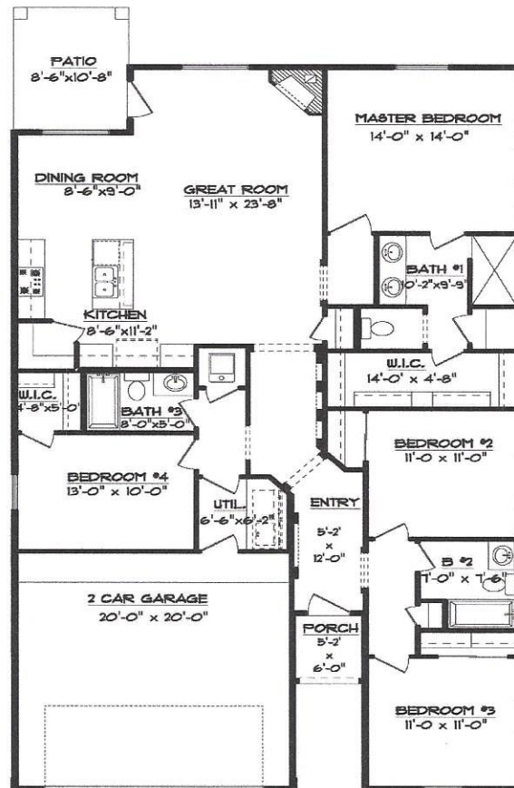
FLOOR PLAN 37'-4" x 62'-4"
