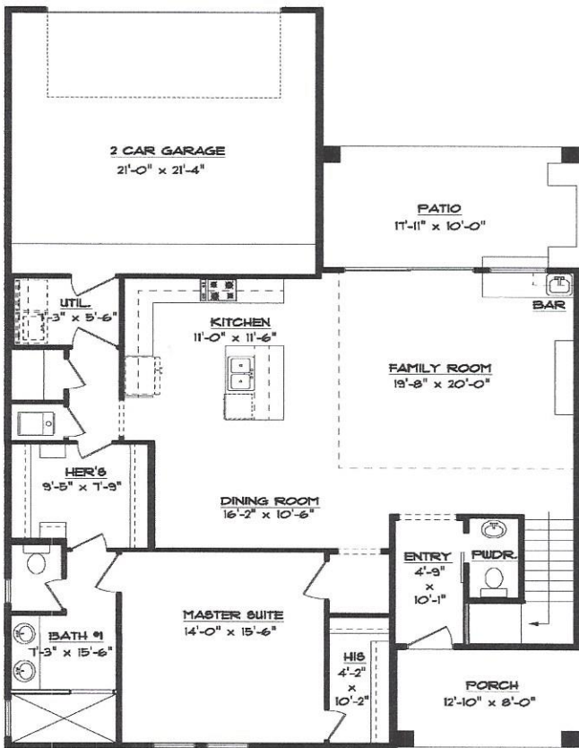
FIRST FLOOR PLAN 39'-6" x 60'-0"
