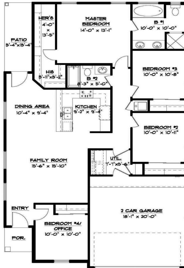
FLOOR PLAN 34'-6" x 58'-8"
