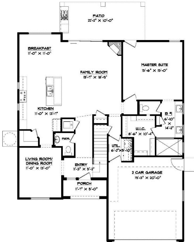
FIRST FLOOR PLAN 43'-0" X 53'-8 1/2"
