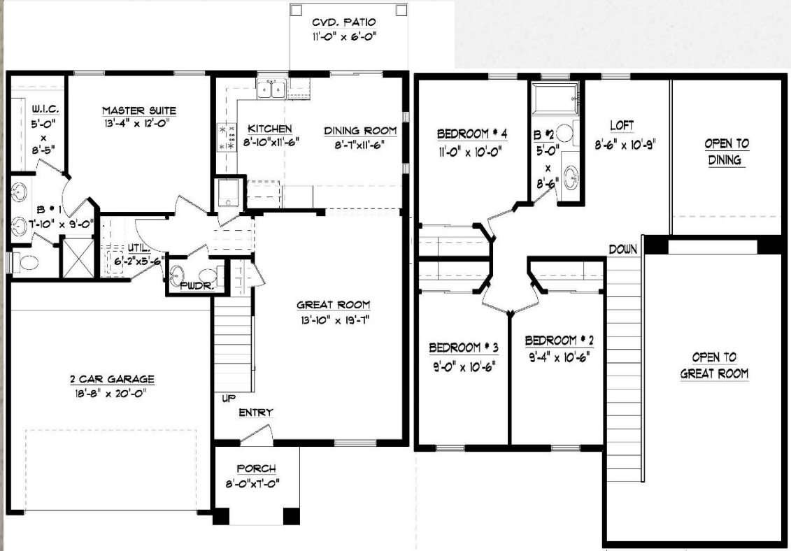
FIRST FLOOR PLAN 37'-4" x 38'-8"
