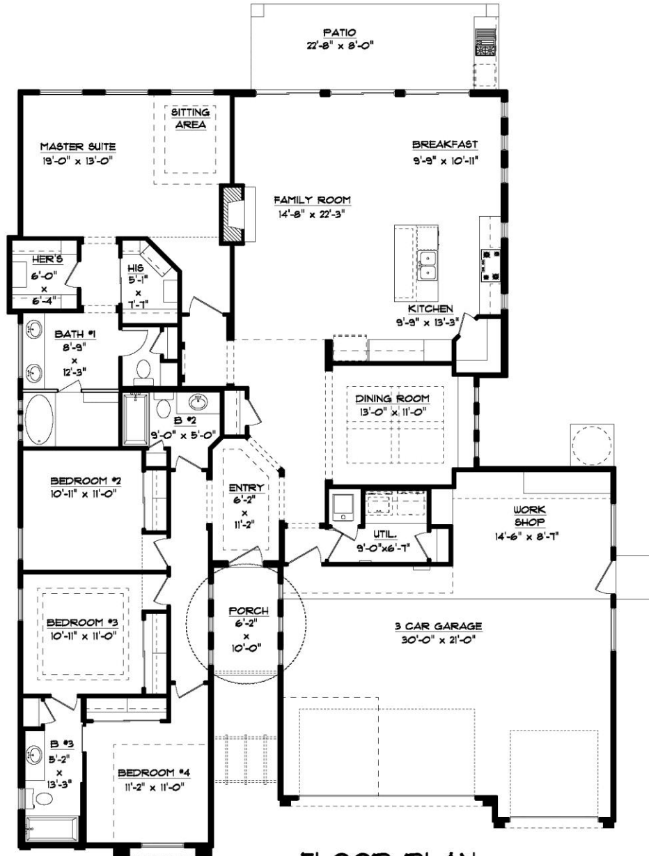
FLOOR PLAN 55'-4 1/2" x 69'-0"
