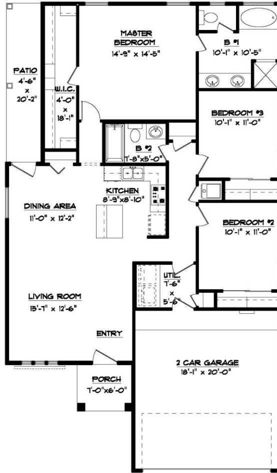
FLOOR PLAN 34'-7" x 59'-0"
