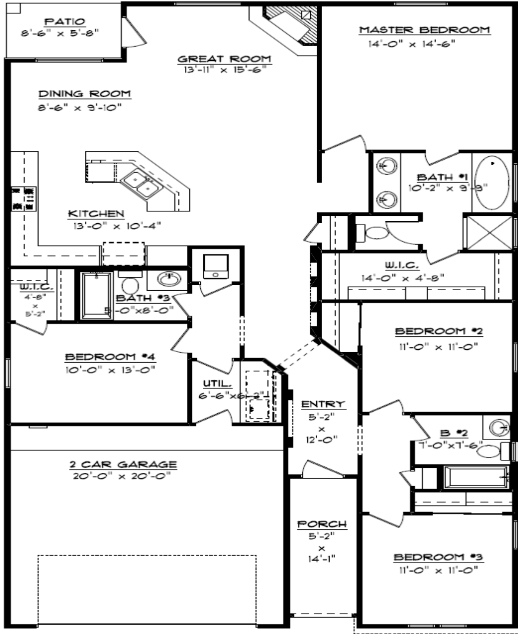
FLOOR PLAN 37'-4" x 62'-10"
